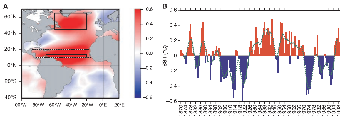
Fig. 2. Atlantic sector of the first rotated EOF of non-ENSO global SST variability for 1870–2000 referred to as the “Atlantic multidecadal mode” (38, 39). (A) Spatial distribution of correlations between local monthly SST anomalies and the modal reconstruction over the indexed region (northern rectangle), the general area where the mode amplitude is the strongest. This distribution has a similar spatial structure to the actual rotated EOF and gives a measure of the local fractional variance (squared temporal correlation) accounted for at each grid point. Dashed lines give north and south boundaries of main development region (MDR) and box (10° to 14°N, 20° to 70°W) is region used to calculate data for Fig. 3. (B) Temporal reconstruction (annual means) of the mode-related variability averaged over the
